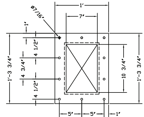
DISCHARGE FLANGE DETAILS
