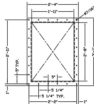
DISCHARGE FLANGE DETAILS
