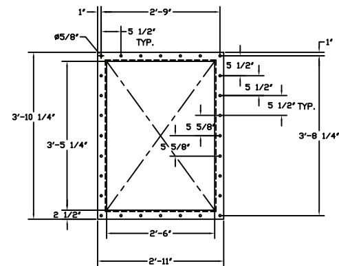
OUTLET FLANGE DETAILS
