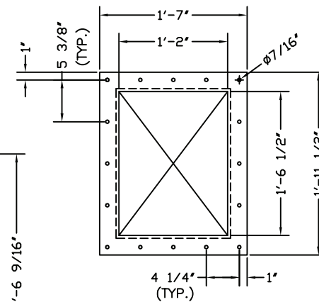
DISCHARGE FLANGE DETAILS
